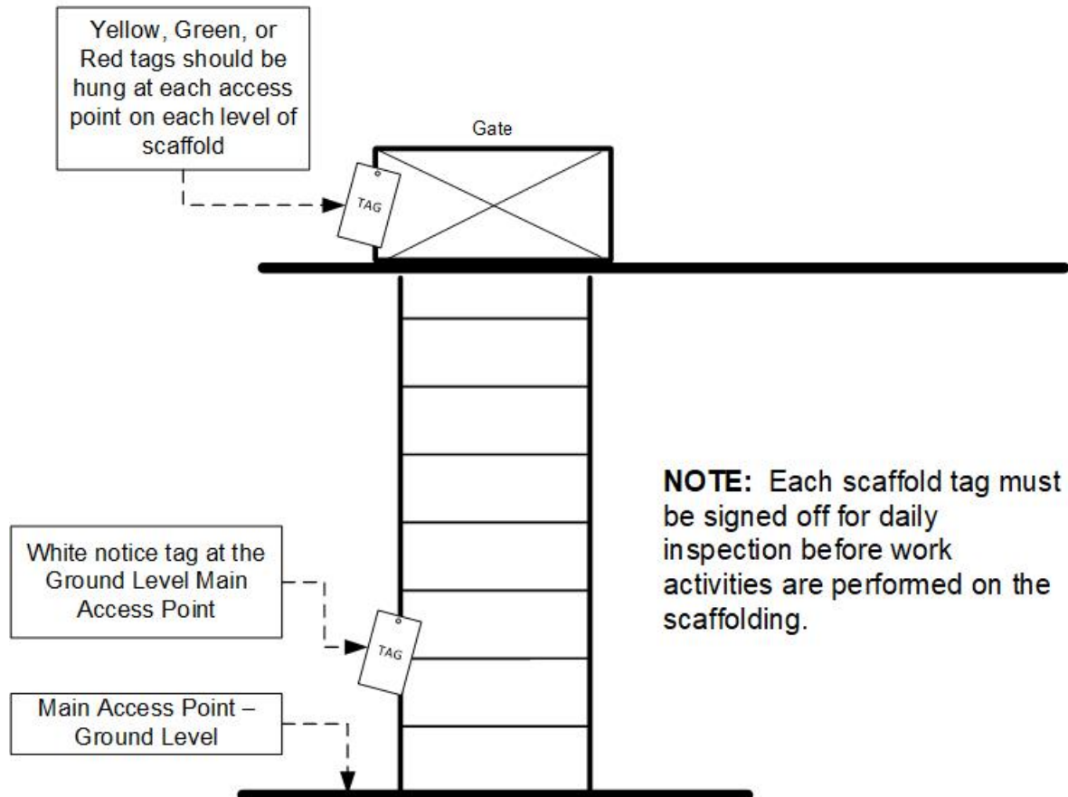
Figure E-2 Guidelines for Tagging Scaffolds
